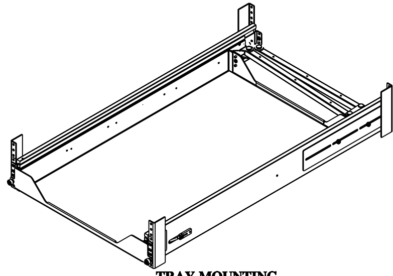
TRAY MOUNTING
