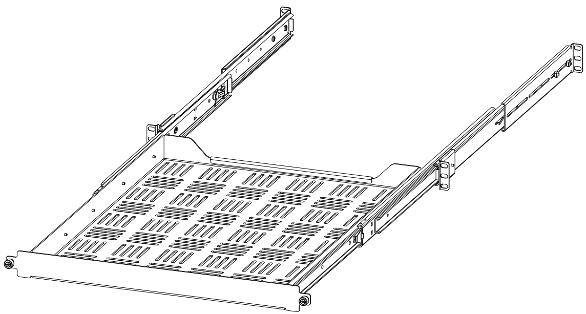
ISO VIEW
